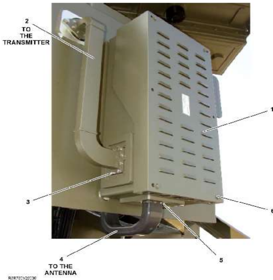
FIGURE 2 : RF UNIT EXTERNAL CONNECTIONS
